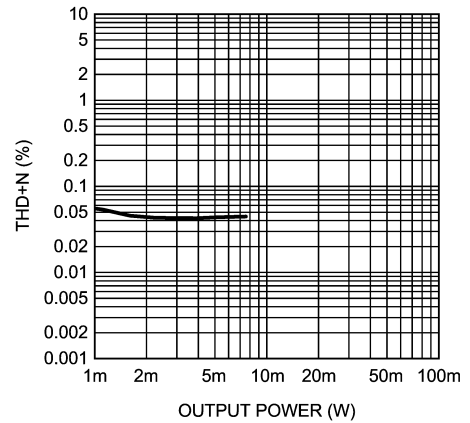
Headphone THD+N vs Output Power
