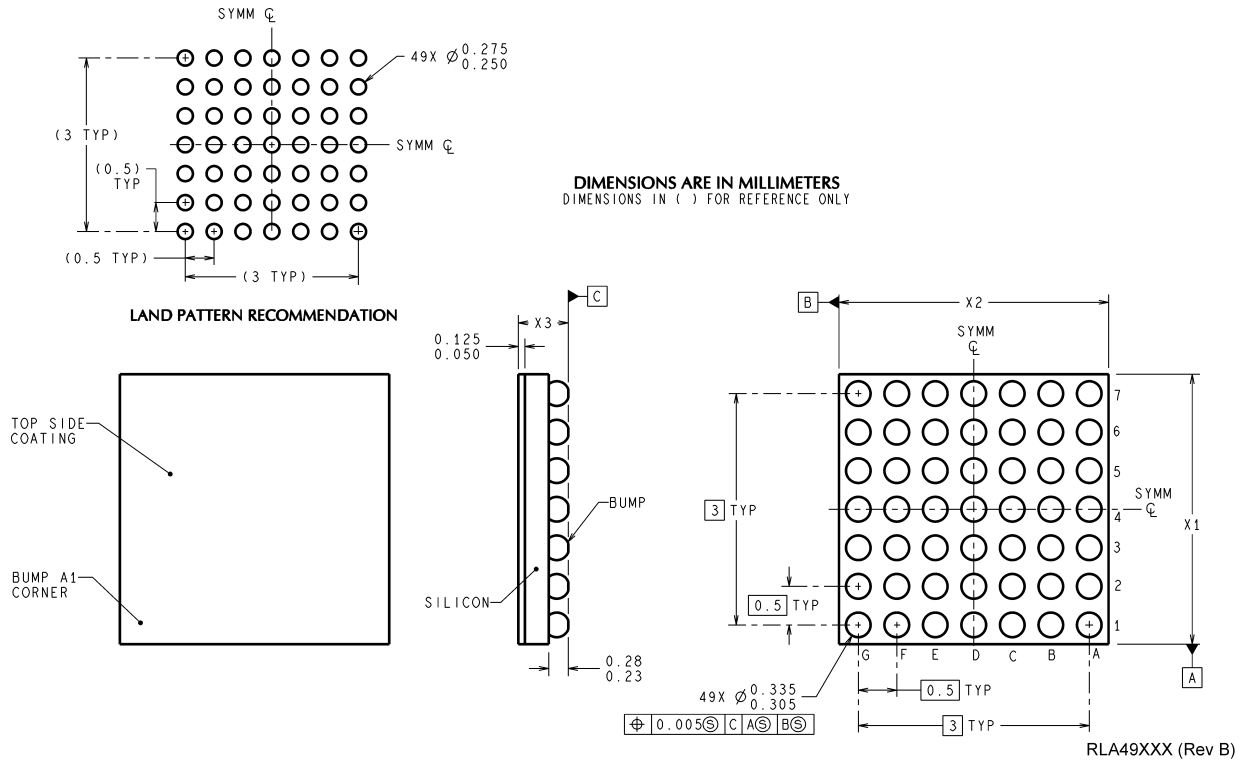
49 Bump micro SMDxt Package Order Number LM4935RL
