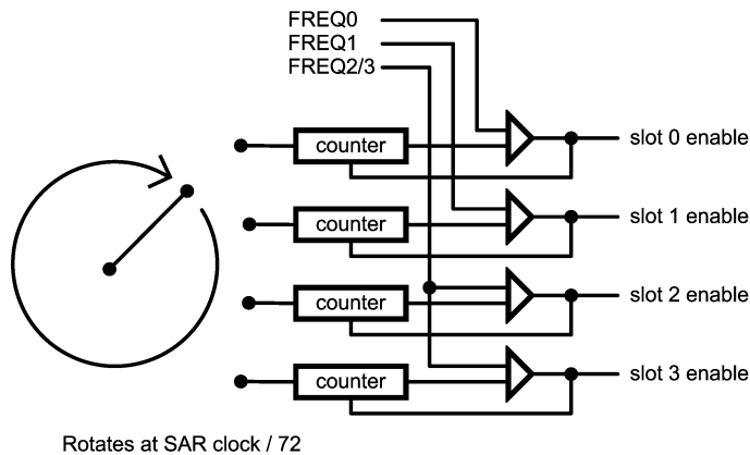
FIGURE 13. Internal SAR Control Signals to SAR Module
