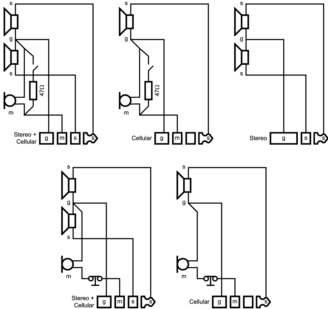
FIGURE 8. Headset Configurations Supported by the LM4935
